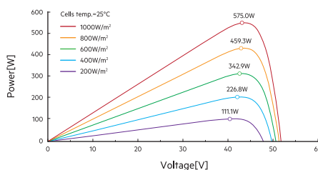
Power-Voltage Curve
